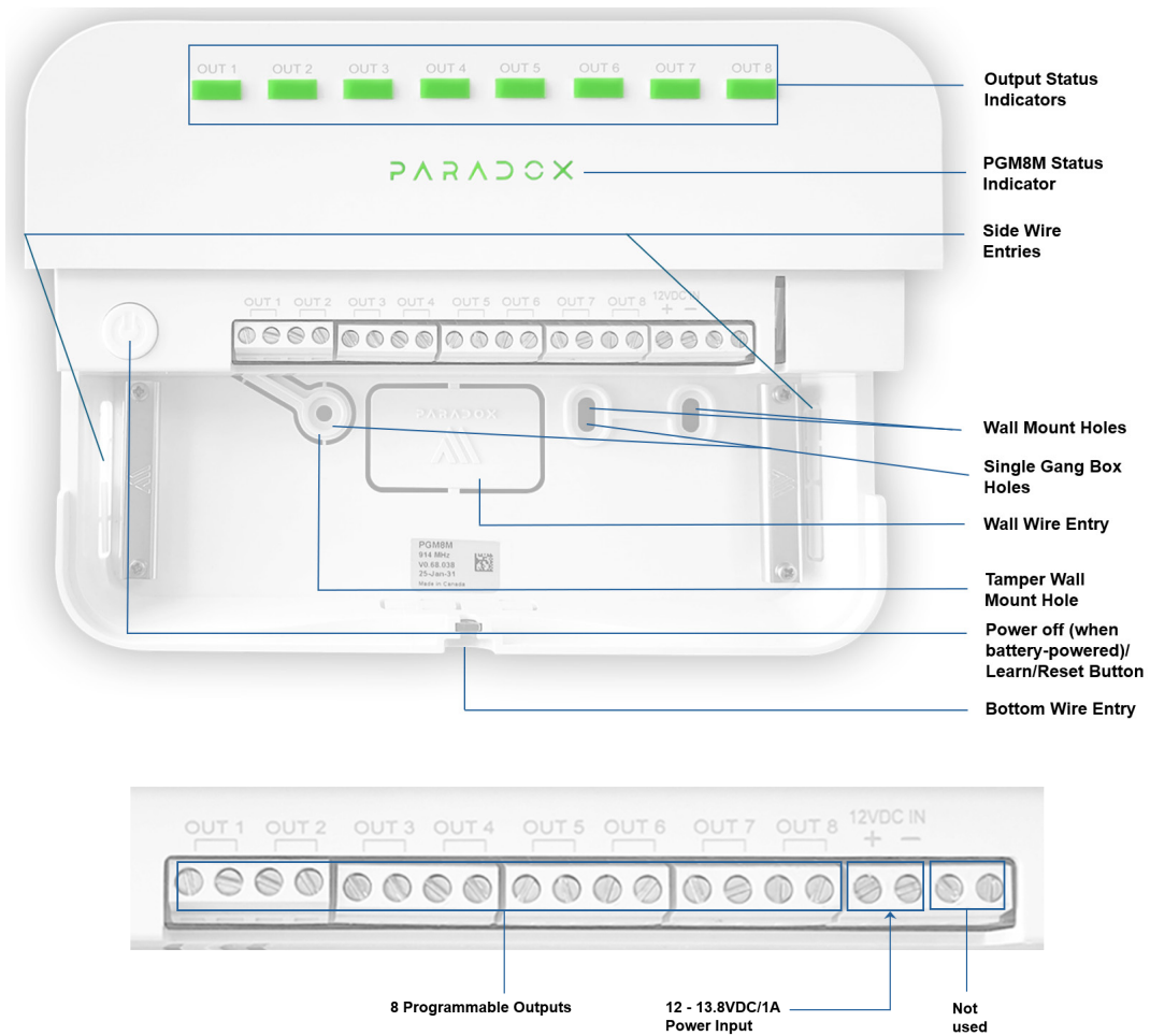
Components of PGM8M
